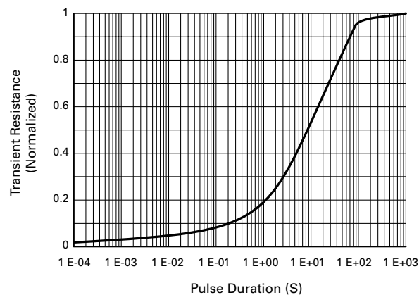
Figure 4. Thermal Response
