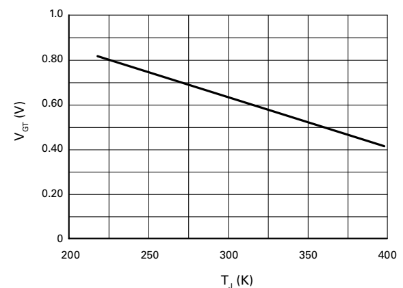
Figure 11. Gate Triggering Voltage vs. T_J
