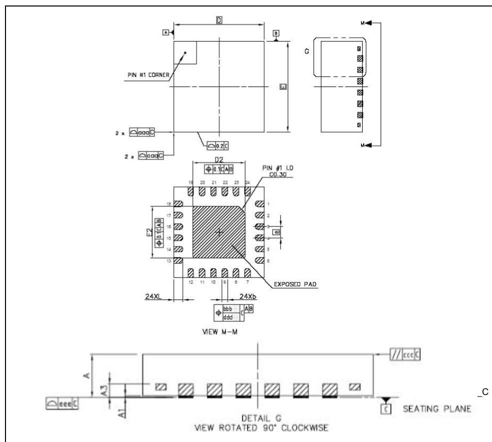
QFPN-24 (4x4x1.8 mm 3 ) Quad Flat Package No lead
