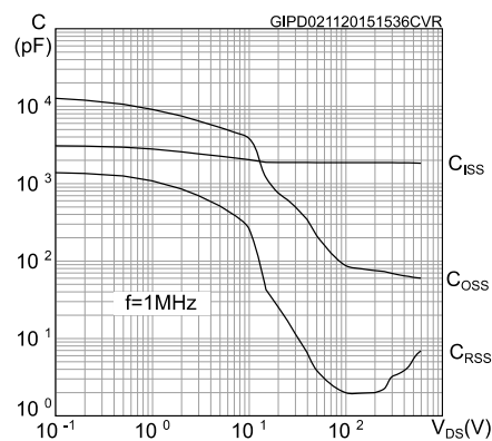
Figure 12: Capacitance variations
