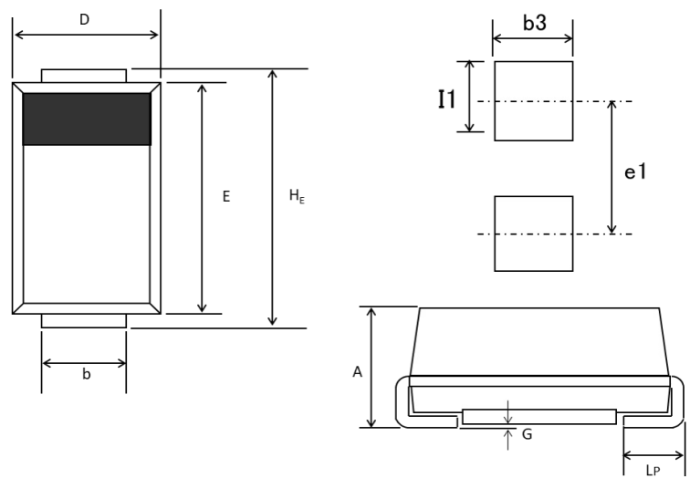
DO-214AC(SMA), (FVDS)
