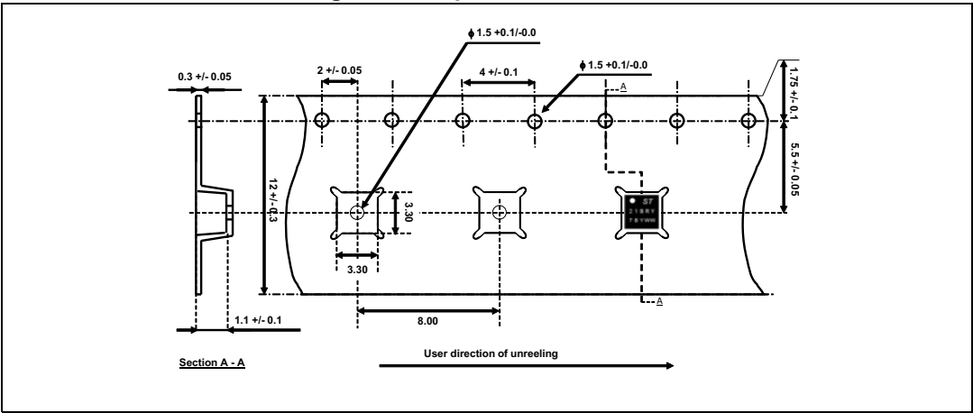
Figure 13. Tape and reel outline
