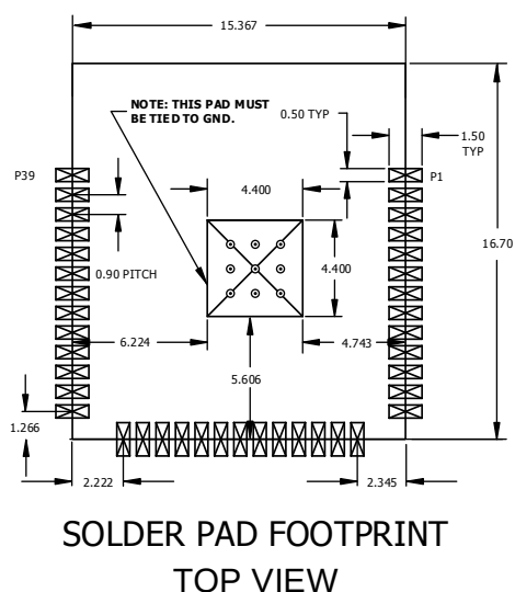
Figure 4-3. ATSAMB11-MR210CA Customer PCB Footprint
