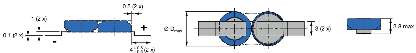
Fig. 7 - Form E2: Surface Mount Flat
