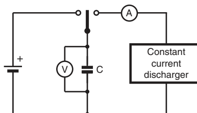
Fig. 16 - Test Circuit for Capacitance Measurement
