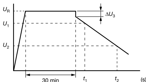
Fig. 15 - Voltage Diagram for Capacitance Measurement
