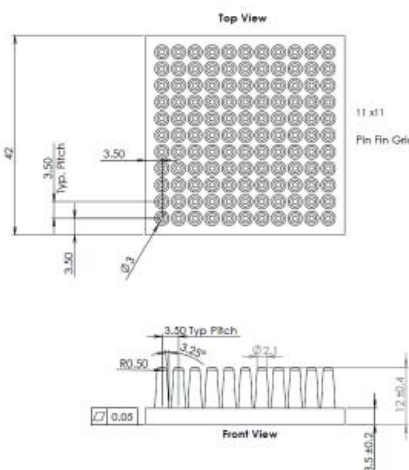
Drawing J: 42x42x12mm
