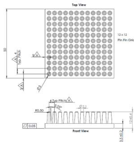
Drawing L: 50x50x12mm
