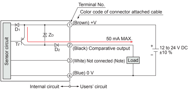
I/O circuit diagram
