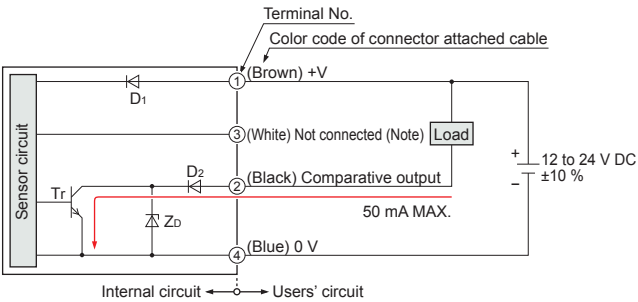
I/O circuit diagram
