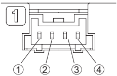
Terminal arrangement diagram
