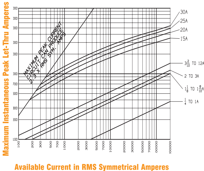
Peak Let-Thru Current Data—ATQR 1/4 to 30, 600 Volts AC
