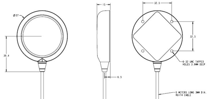
Dimensions (mm)
