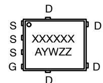
DFN5 CASE 506EZ
