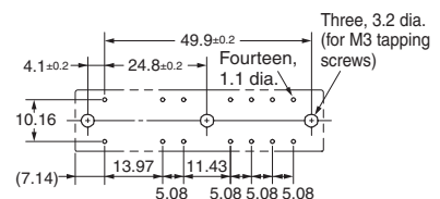
G7SA-4A2B Mounted
