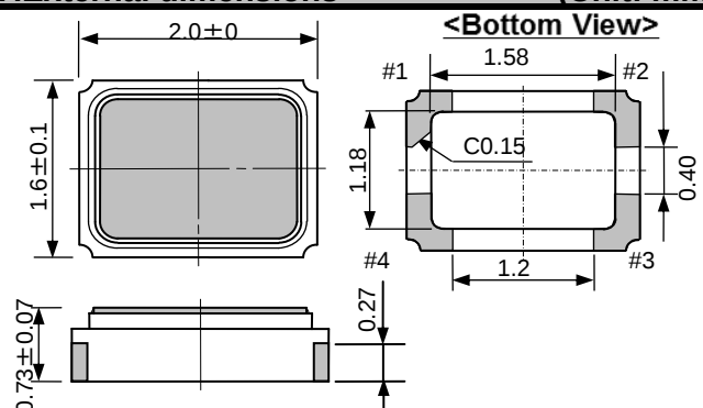
Pin map
