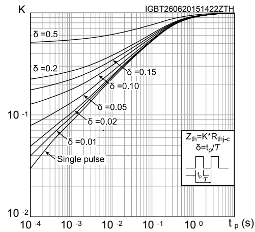
Figure 17. Thermal impedance
