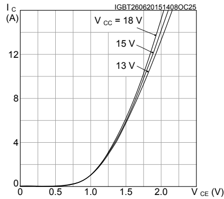
Figure 11. Output characteristics
