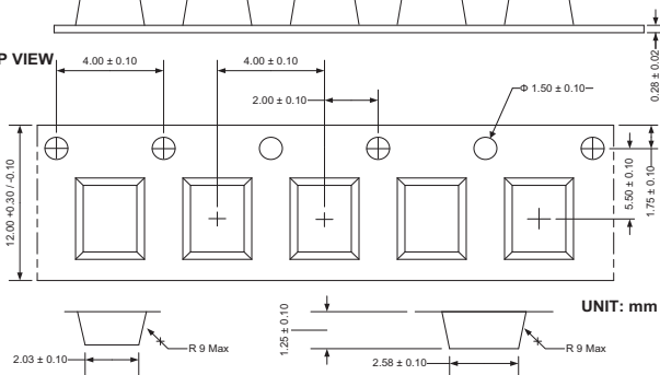
Fig. 15 - VEML6070 A3OP Package Carrier Tape
