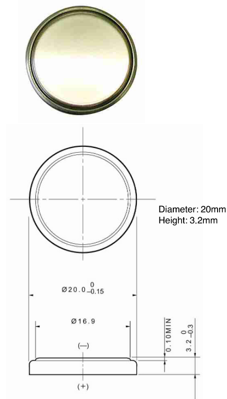
Dimension Drawing
