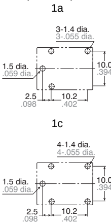
PC board pattern (Bottom view)
