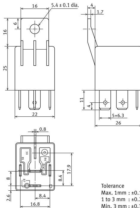
External dimensions
