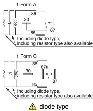
Schematic (Bottom view)
