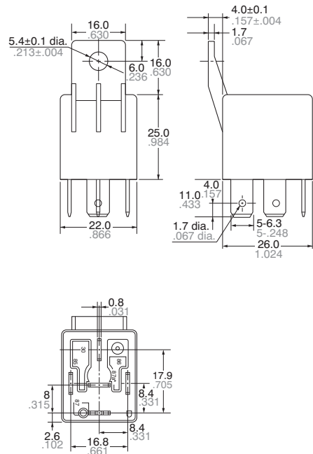
External dimensions
