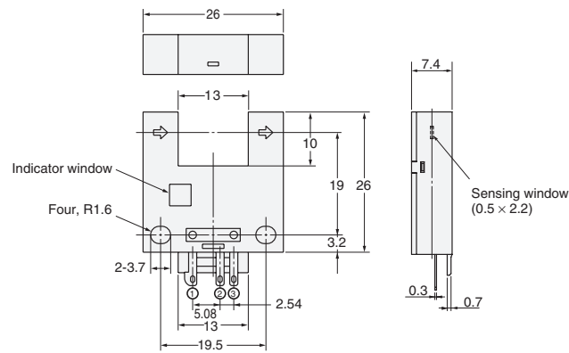
Terminal Arrangement
