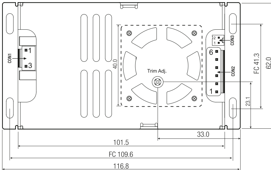
Dimension Drawing (mm) Top View
