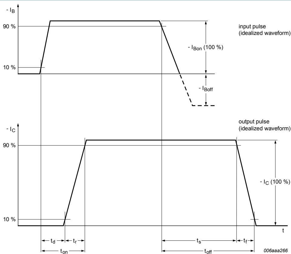
Fig. 22. TR2 (PNP): BISS transistor switching time definition
