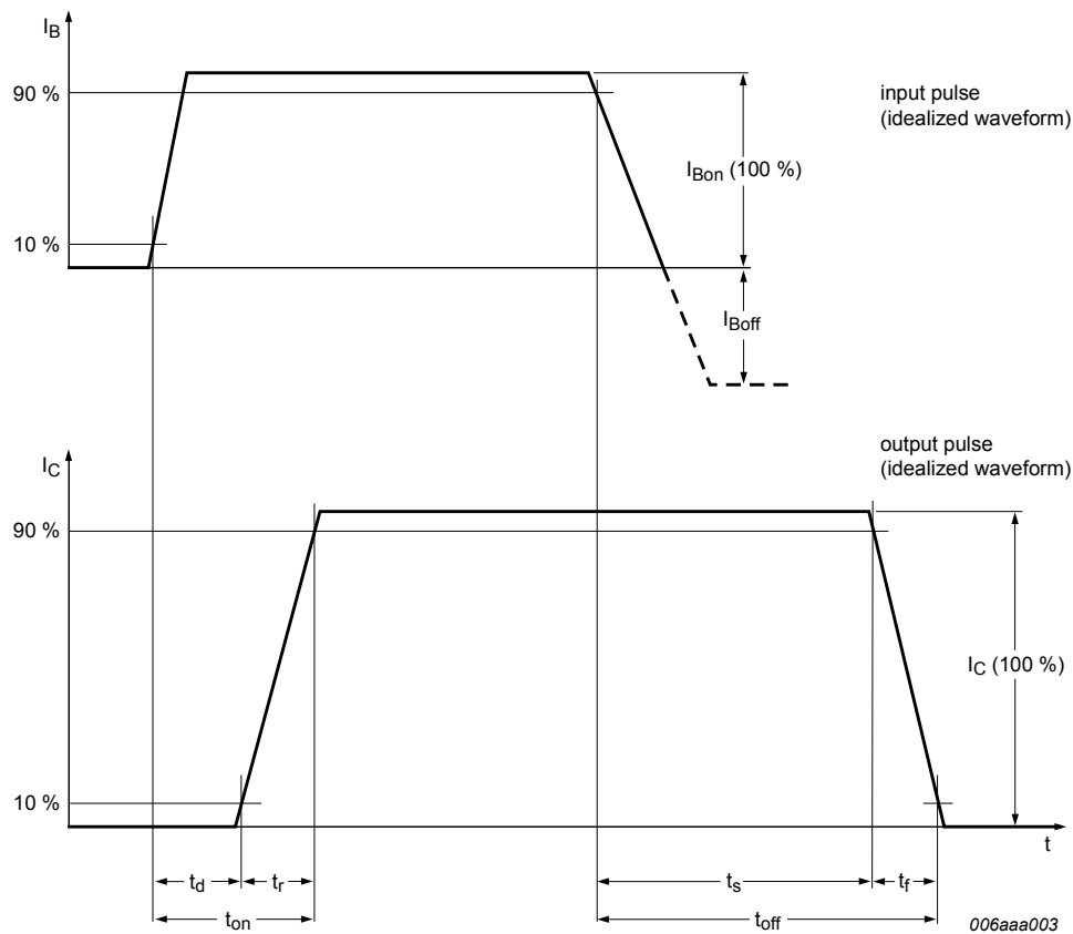
Fig. 12. BISS transistor switching time definition
