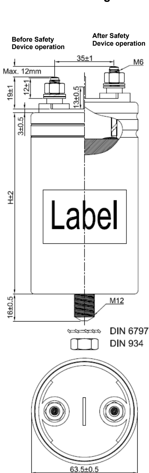
Figure 2: Series B32361
