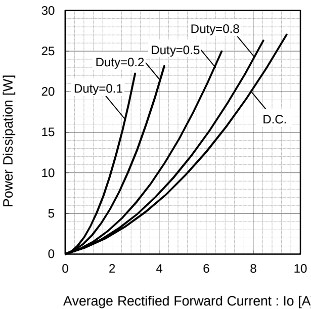
Fig.8 Io-Pf Characteristics
