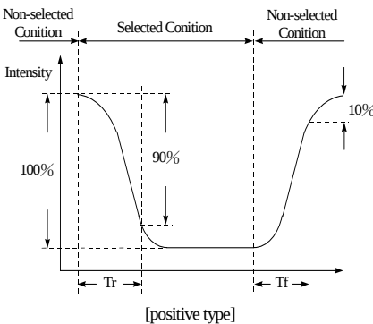
Definition of Response Time ( Tr , Tf )
