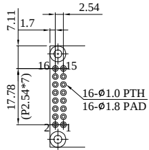
PIN DETAIL
