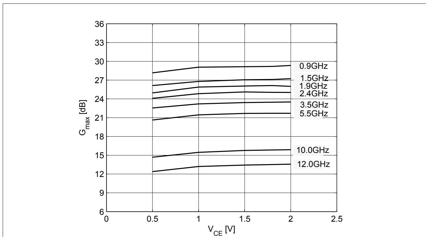
Figure 15 Maximum power gain G_{\max} = f(V_{CE}) , I_C = 10 \text{ mA} , f = \text{parameter in GHz}
