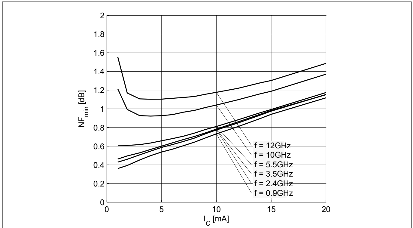
Figure 20 Noise figure NF_{min} = f(I_C) , V_{CE} = 1.8 V, Z_S = Z_{S,opt} , f = parameter in GHz
