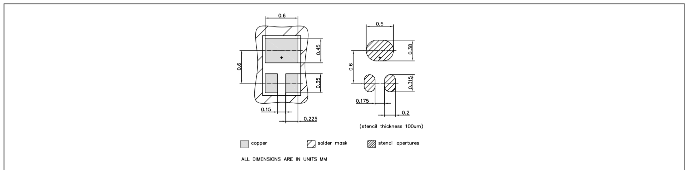
Figure 23 Foot print
