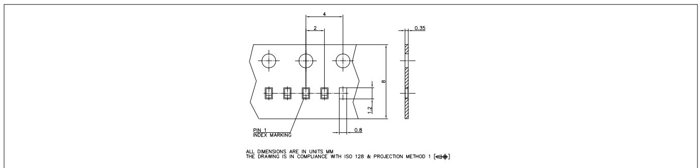
Figure 25 Tape dimensions
