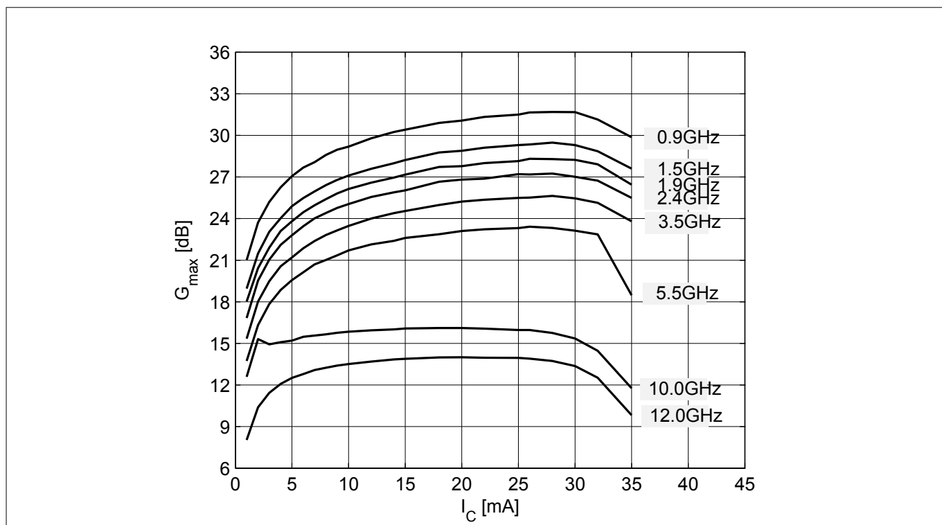
Figure 14 Maximum power gain G_{\max} = f(I_C) , V_{CE} = 1.8 \text{ V} , f = \text{parameter in GHz}
