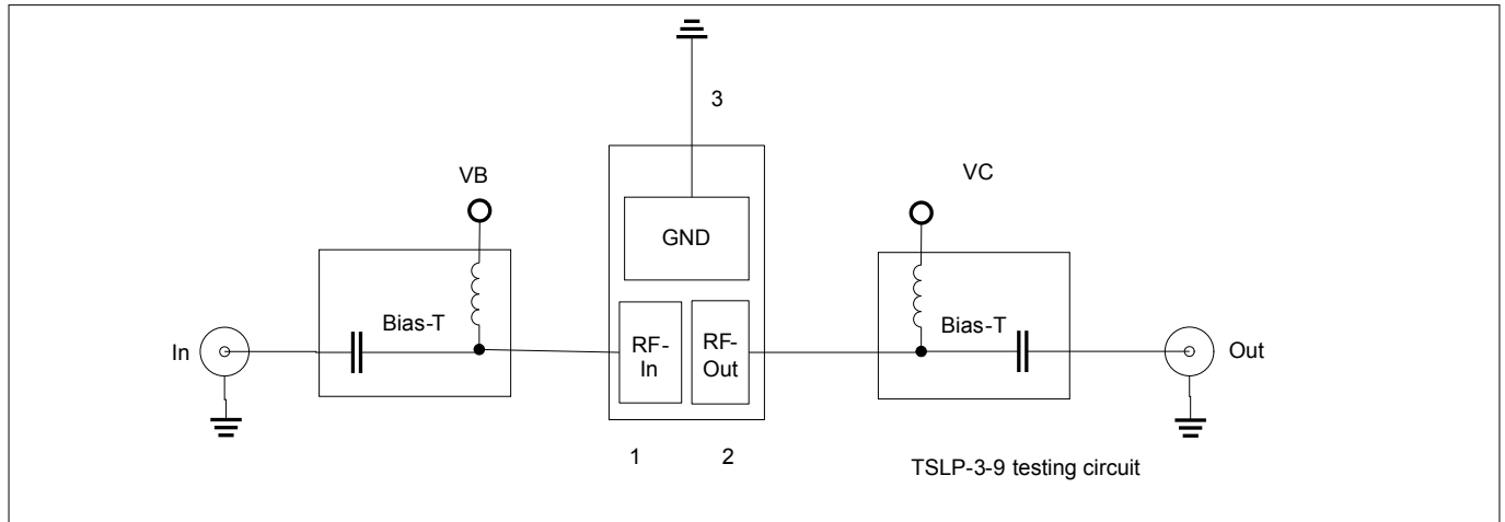
Figure 2 Testing circuit
