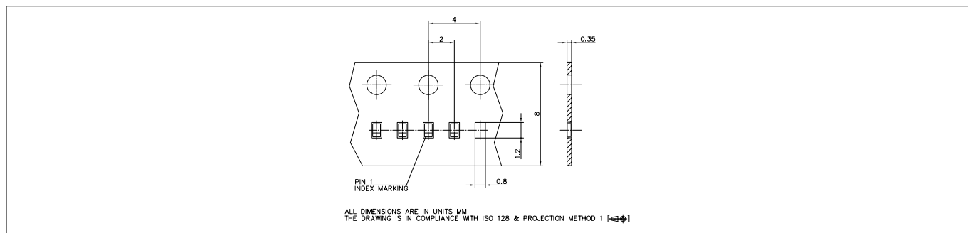
Figure 25 Tape dimensions
