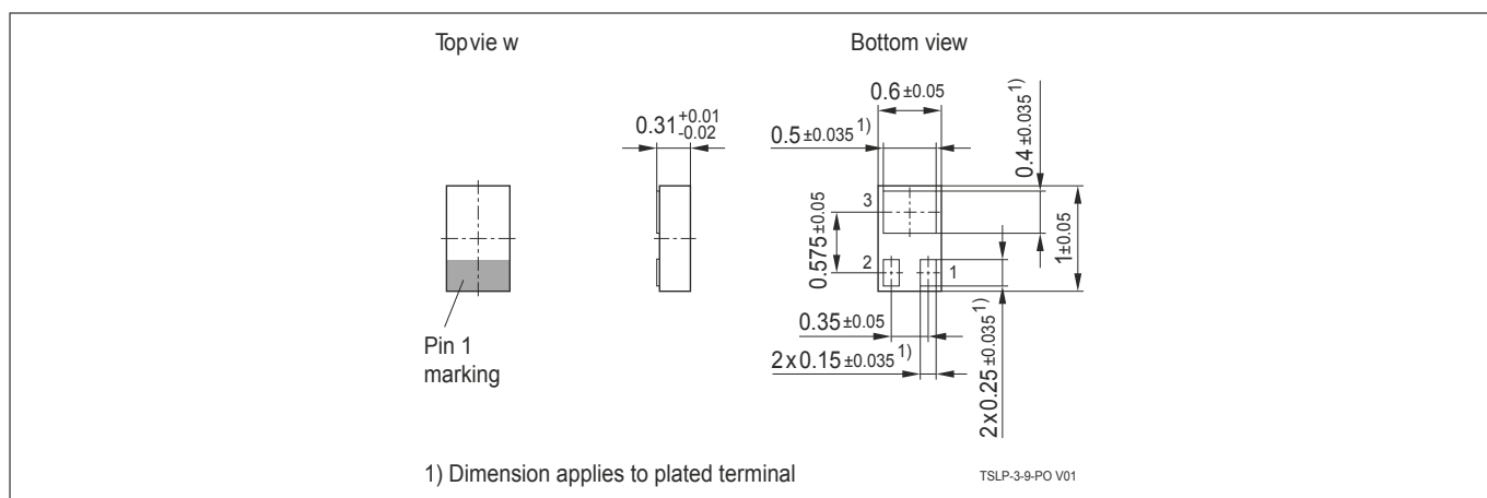
Figure 22 Package outline (dimension in mm)
