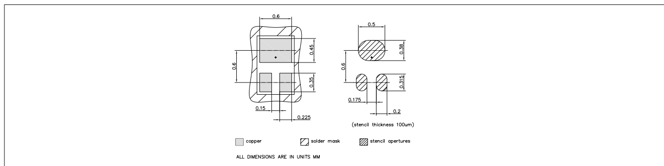
Figure 23 Foot print
