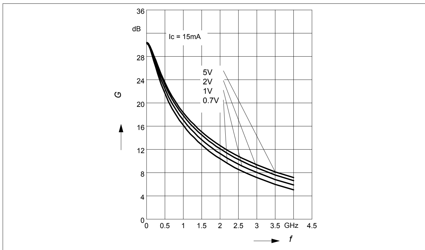
Figure 6 Transducer Gain IS_{21}I^2 = f(f) , I_C = 15 mA, V_{CE} = \text{parameter}
