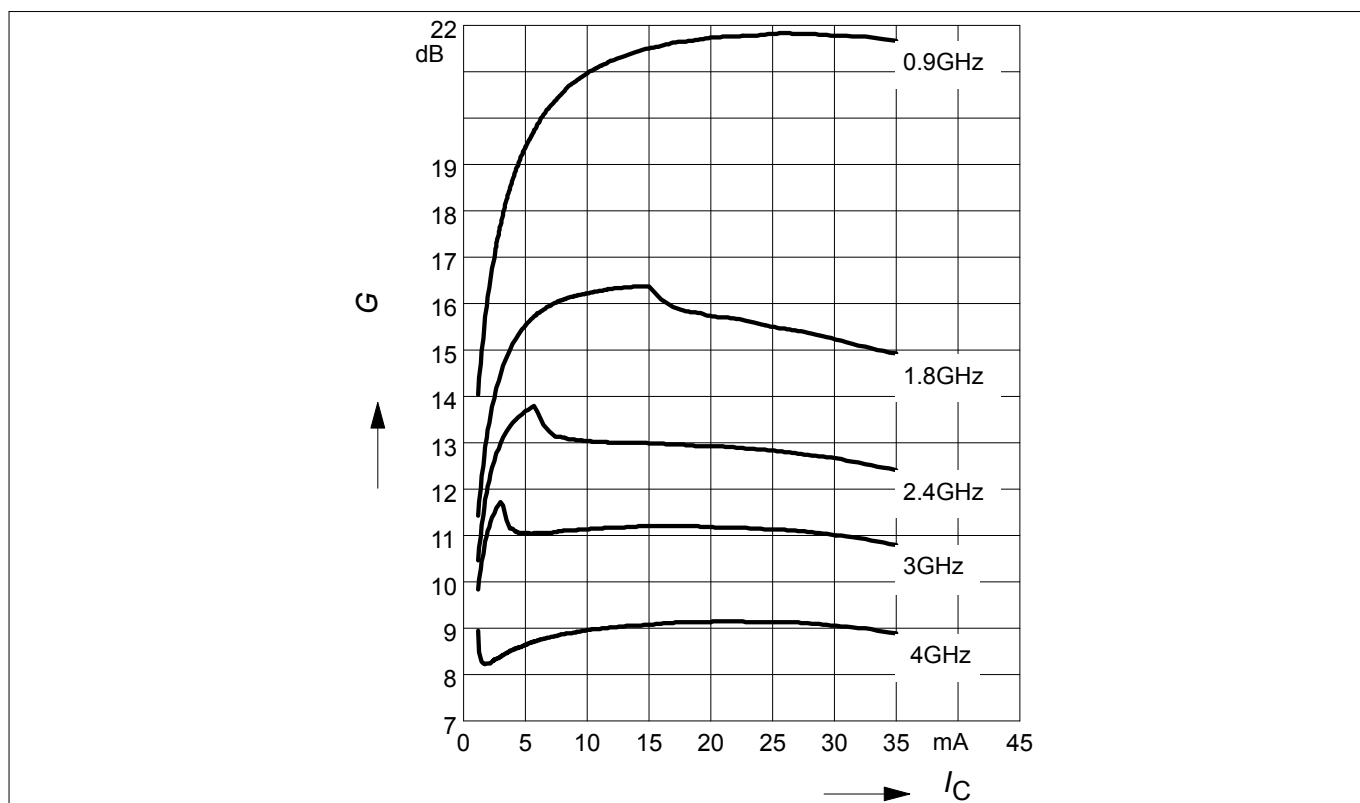
Figure 10 Maximum power gain G_{max} = f(I_C) , V_{CE} = 3 V, f = \text{parameter in GHz}
