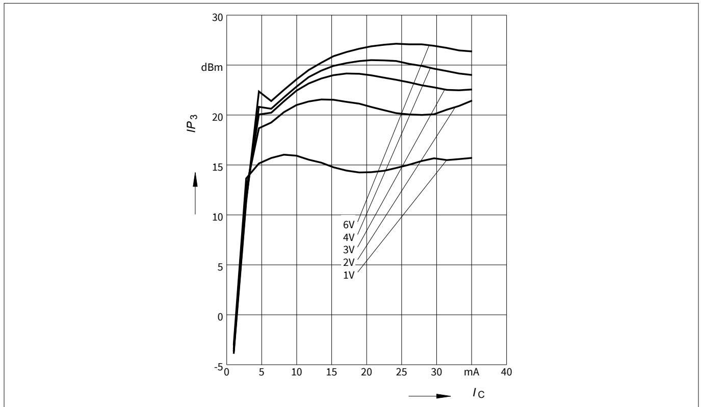
Figure 4 3rd order intercept point OIP_3 = f(I_C) , Z_S = Z_L = 50 \Omega , V_{CE} , f = 1.8 GHz, V_{CE} = \text{parameter}
