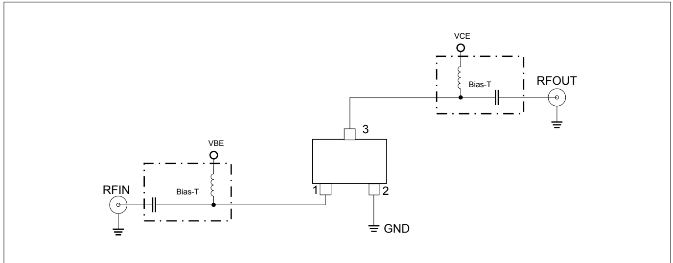
Figure 2 Testing circuit
