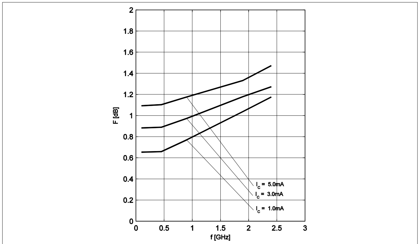
Figure 12 Noise figure NF_{min} = f(f) , V_{CE} = 1.5 V, Z_S = Z_{S,opt} , I_C = 1 / 3 / 5 mA
