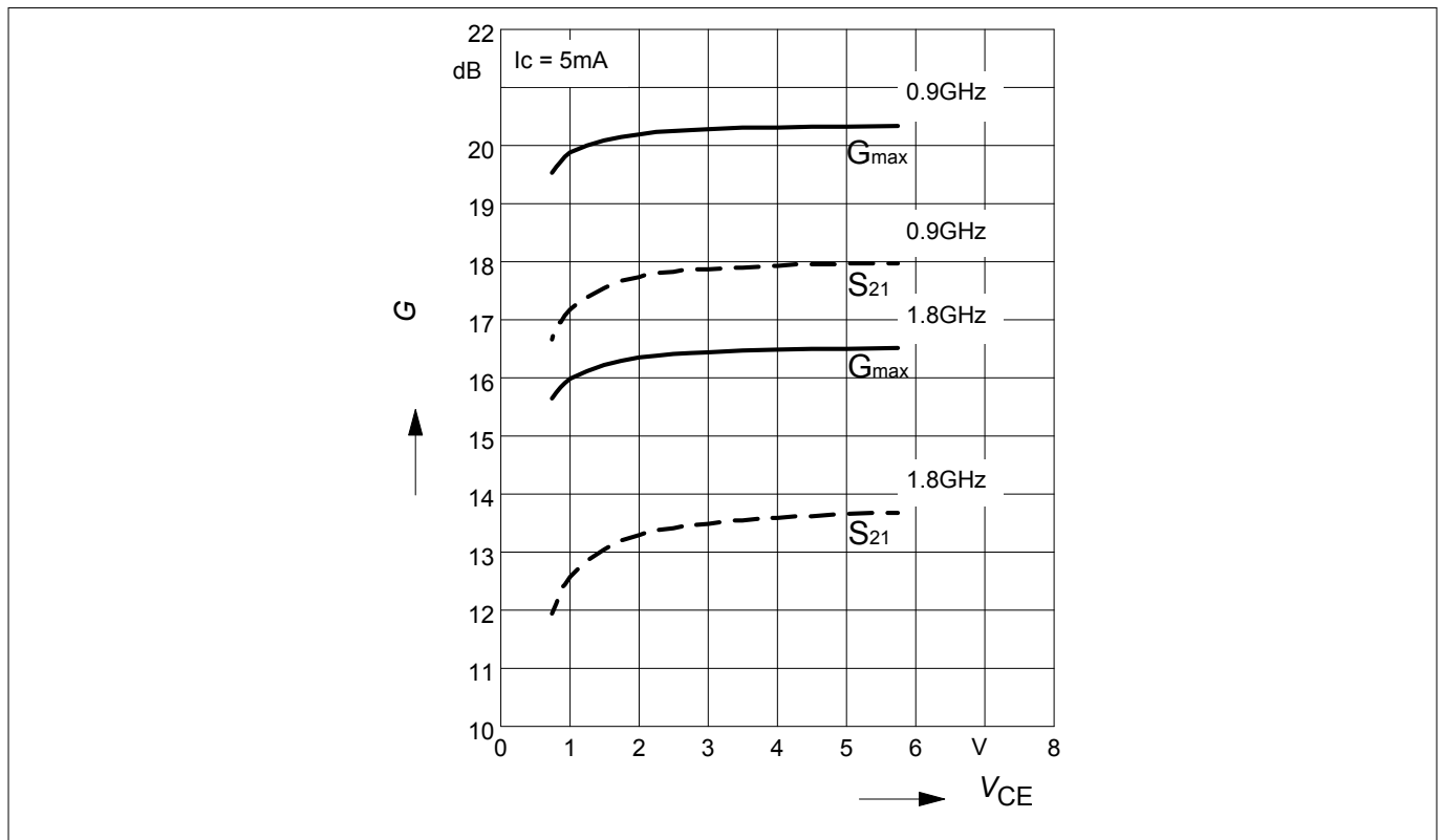
Figure 10 Maximum power gain G_{\max} = f(V_{CE}) , transducer gain IS_{21}I^2 = f(V_{CE}) , I_C = 5\text{ mA} , f = \text{parameter in GHz}
