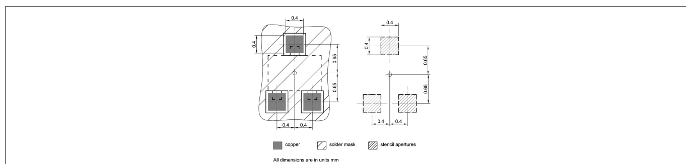
Figure 16 Foot print
