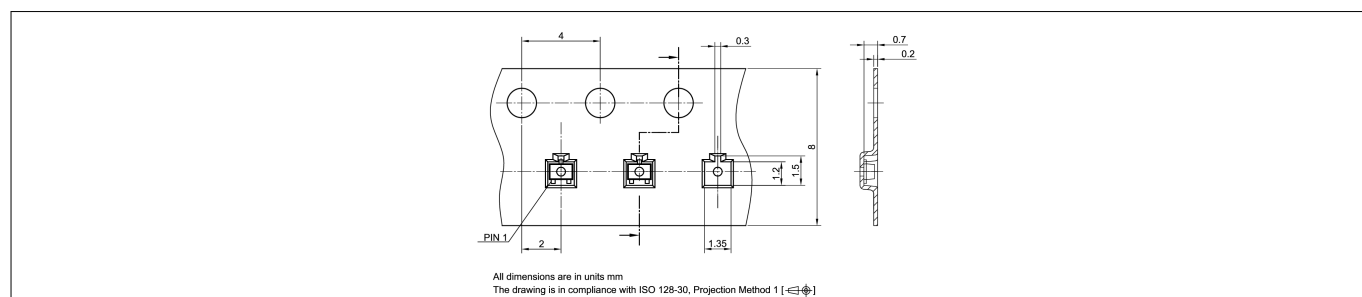
Figure 18 Tape information
