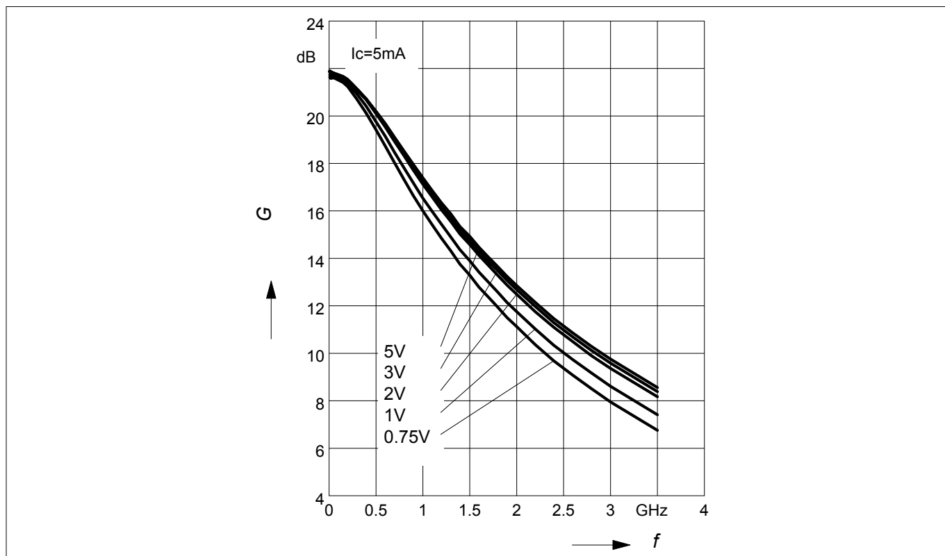
Figure 8 Transducer gain IS_{21}I^2 = f(f) , I_C = 5\text{ mA} , V_{CE} = \text{parameter}
