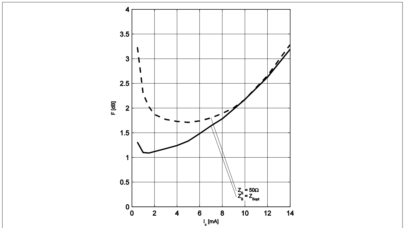
Figure 14 Noise figure NF_{\min} = f(I_c) , Z_S = Z_{S,\text{opt}} , NF_{50} = f(I_c) , Z_S = 50\Omega , V_{CE} = 3\text{ V} , f = 1.9\text{ GHz}
