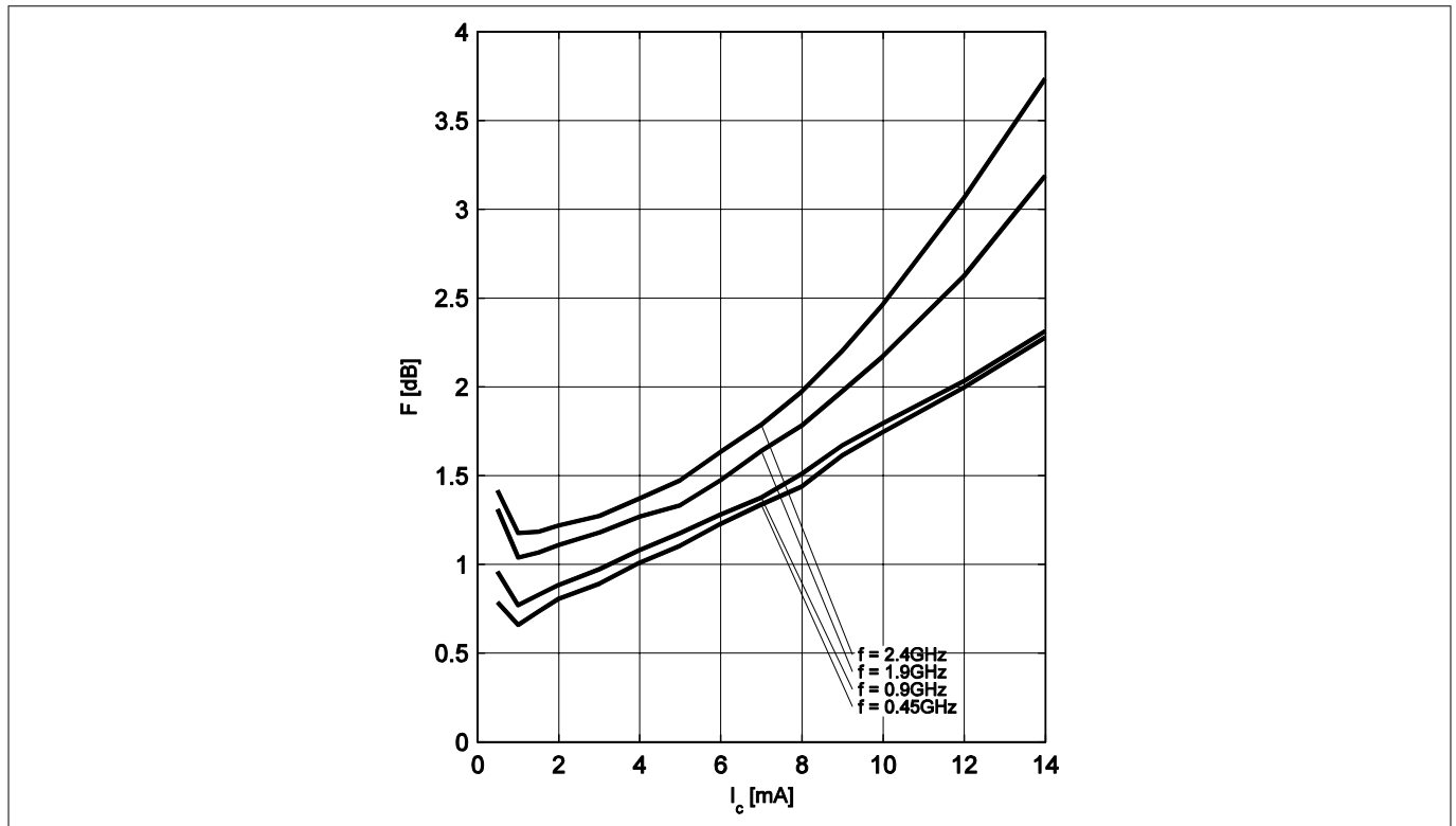
Figure 13 Noise figure NF_{\min} = f(I_c) , V_{CE} = 1.5\text{ V} , Z_S = Z_{S,\text{opt}} , f = \text{parameter in GHz}
