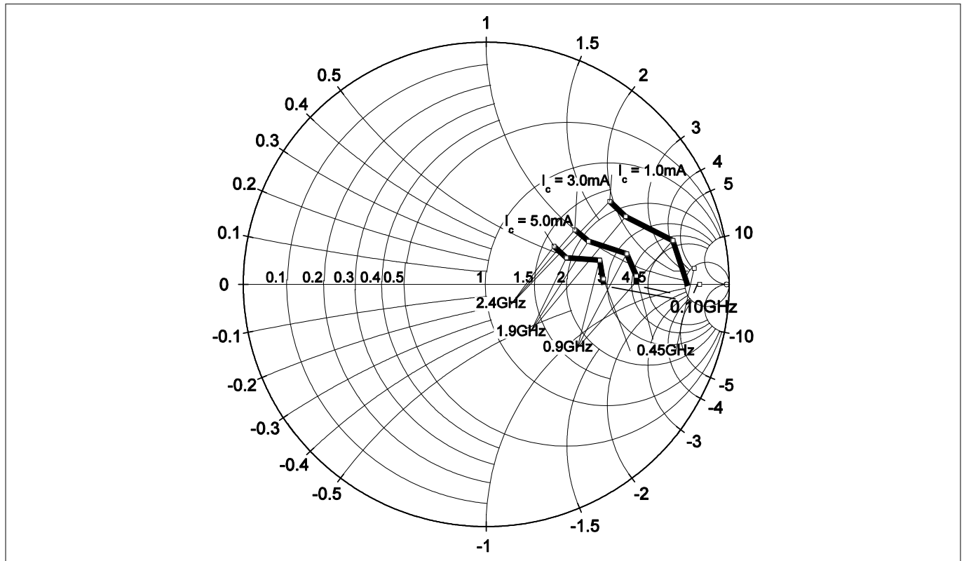
Figure 11 Source impedance for minimum noise figure Z_{S,opt} = f(f) , V_{CE} = 1.5 V, I_C = \text{parameter}
