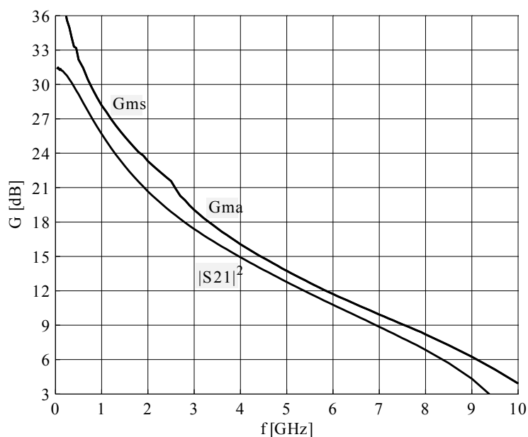
Figure 10 Gain G_{ma} , G_{ms} , |S_{21}|^2 = f(f) , V_{CE} = 2.5\text{ V} , I_C = 15\text{ mA}
