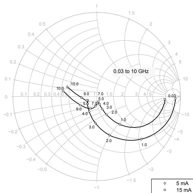
Figure 16 Input reflection coefficient S_{11} = f(f) , V_{CE} = 2.5 \text{ V} , I_C = 5 / 15 \text{ mA}
