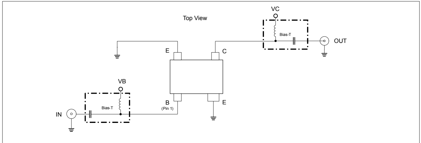
Figure 2 Testing circuit
