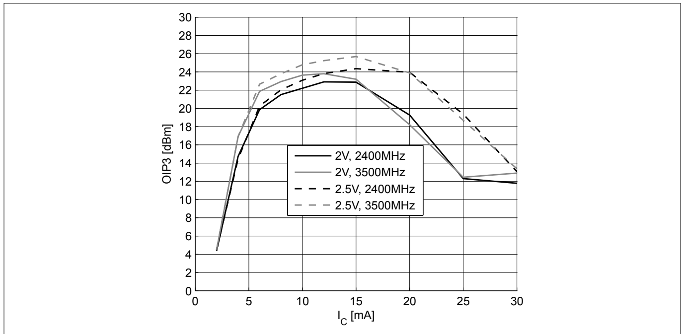
Figure 13 3rd order intercept point at output OIP_3 = f(I_C) , Z_S = Z_L = 50 \Omega , V_{CE} , f = parameter
