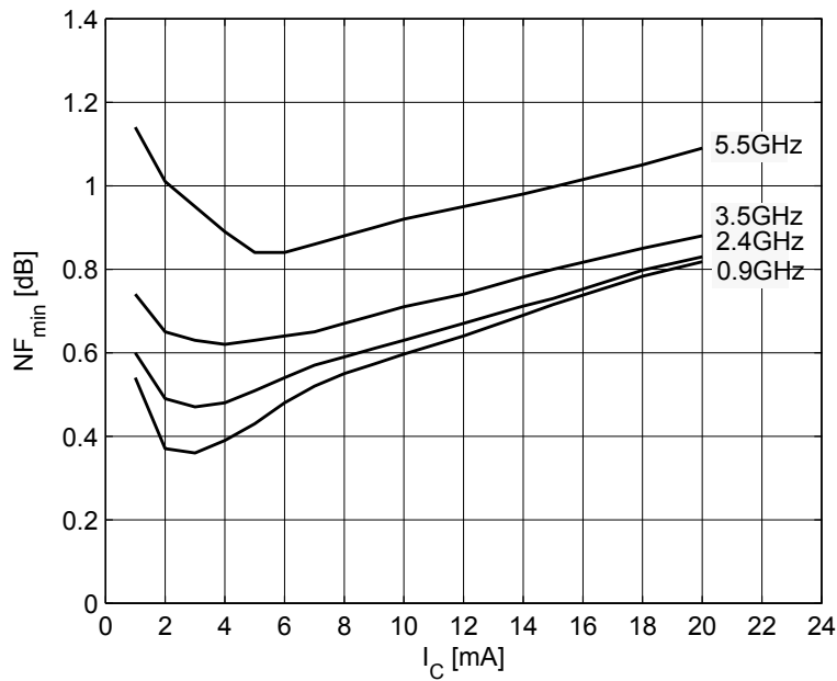
Figure 20 Noise figure NF_{min} = f(I_C) , V_{CE} = 2.5 V, Z_S = Z_{S,opt} , f = \text{parameter}
