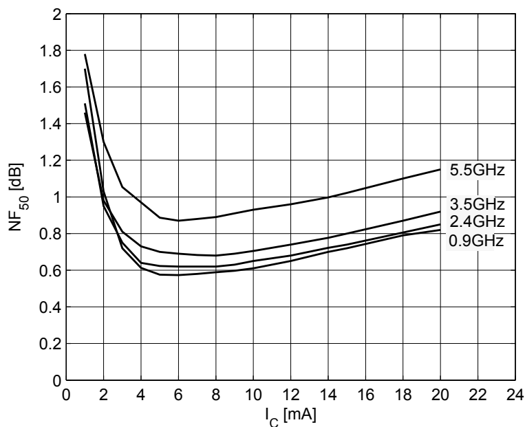
Figure 21 Noise figure NF_{50} = f(I_C) , V_{CE} = 2.5 V, Z_S = 50 \Omega , f = \text{parameter}
