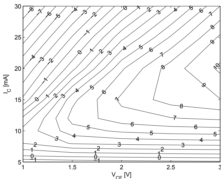
Figure 14 Compression point at output OP_{1dB} [dBm] = f(I_C, V_{CE}) , Z_S = Z_L = 50 \Omega , f = 3.5 \text{ GHz}
