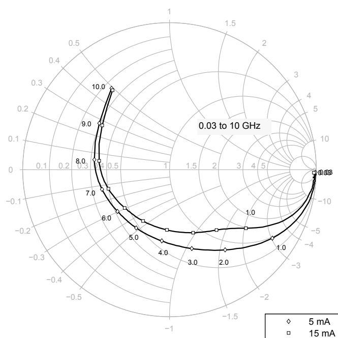
Figure 17 Output reflection coefficient S_{22} = f(f) , V_{CE} = 2.5 \text{ V} , I_C = 5 / 15 \text{ mA}
