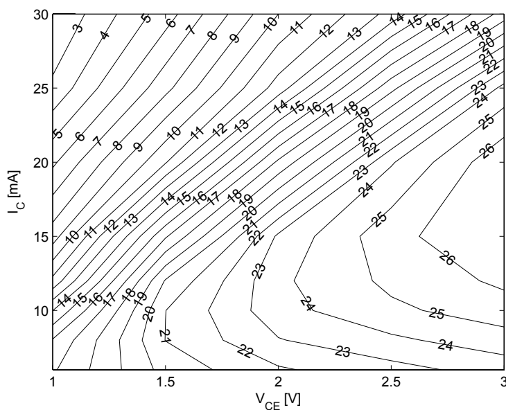
Figure 15 3rd order intercept point at output OIP_3 [dBm] = f(I_C, V_{CE}) , Z_S = Z_L = 50 \Omega , f = 3.5 \text{ GHz}
