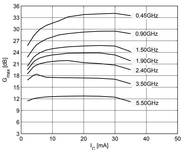
Figure 11 Maximum power gain G_{max} = f(I_C) , V_{CE} = 2.5\text{ V} , f = \text{parameter}
