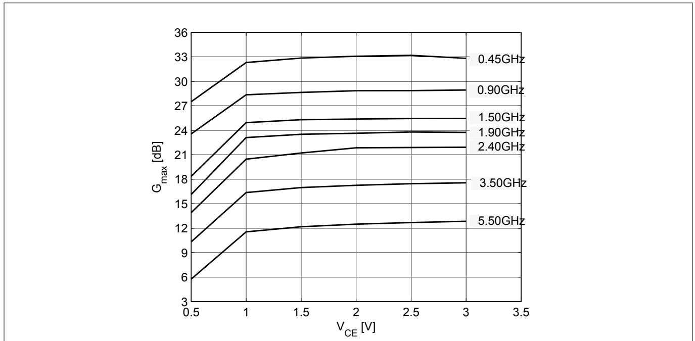
Figure 12 Maximum power gain G_{max} = f(V_{CE}) , I_C = 15 mA, f = parameter
