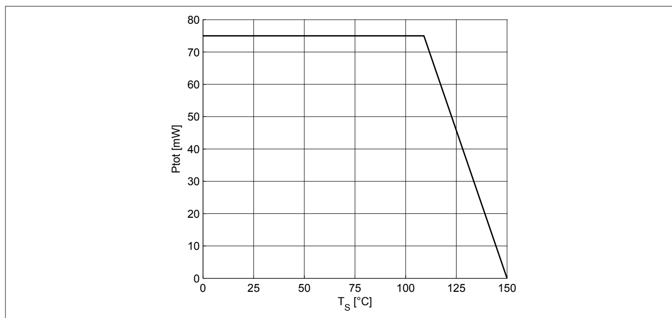
Figure 1 Total power dissipation P_{tot} = f(T_s)
