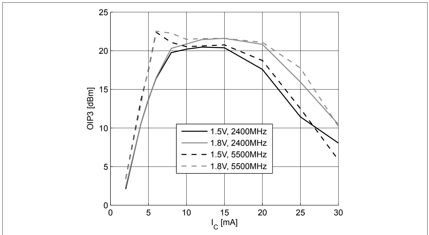
Figure 9 3rd order intercept point at output OIP_3 = f(I_C) , Z_S = Z_L = 50 \Omega , V_{CE} , f = \text{parameter}
