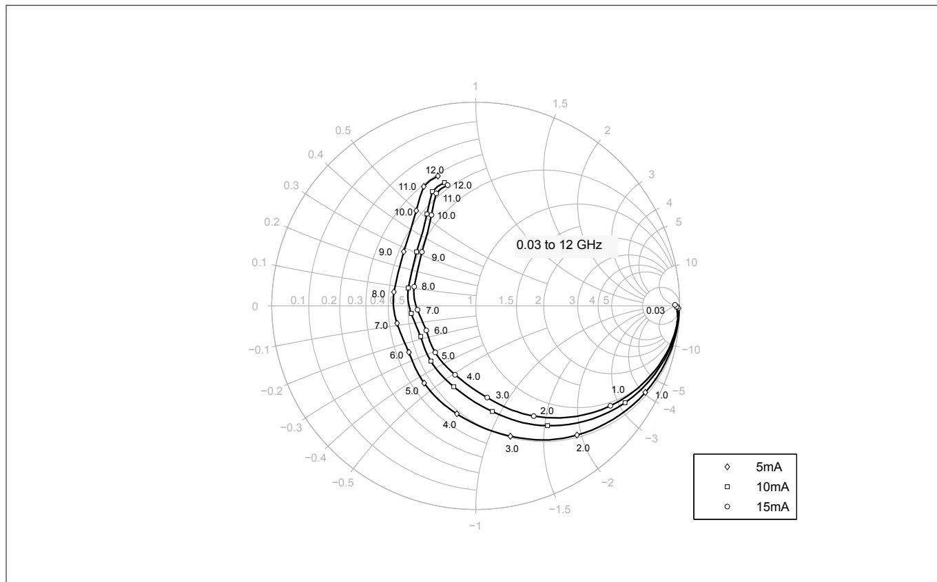
Figure 18 Output reflection coefficient S_{22} = f(f) , V_{CE} = 1.8 \text{ V} , I_C = 5 / 10 / 15 \text{ mA}
