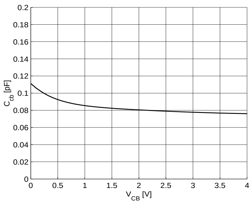
Figure 5-9 Collector Base Capacitance C_{CB} = f(V_{CB}) , f = 1 MHz
