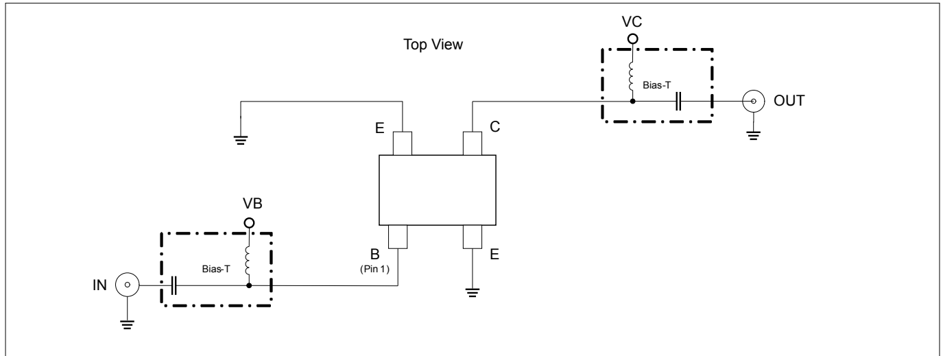
Figure 2 Testing circuit
