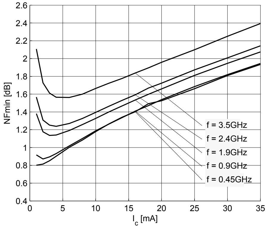
Figure 21 Noise figure NF_{min} = f(I_c) , V_{CE} = 3\text{ V} , Z_S = Z_{S,opt} , f = \text{parameter in GHz}
