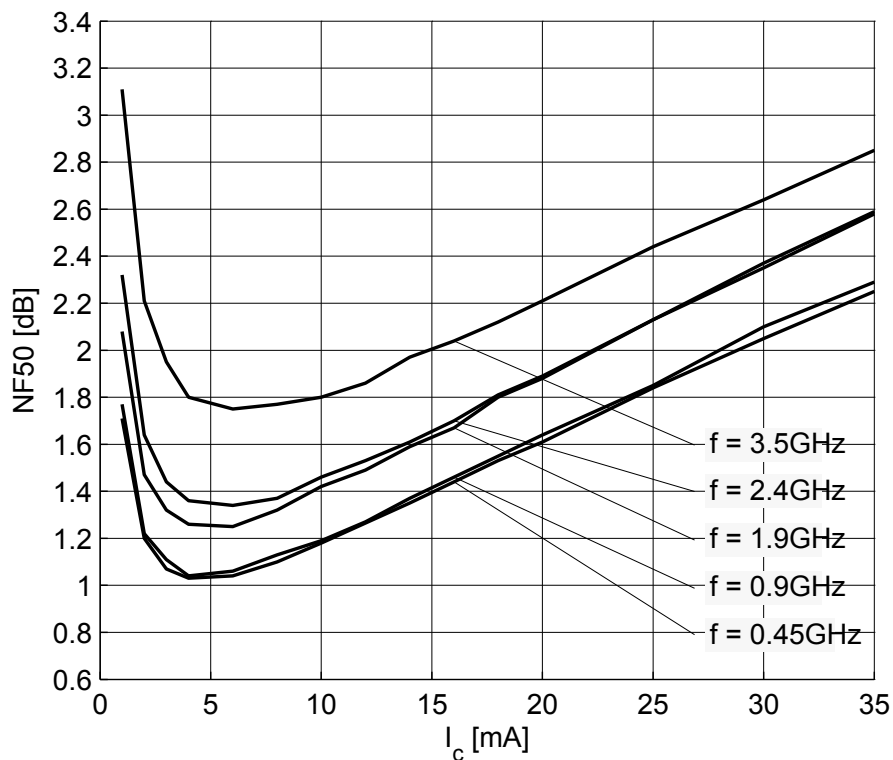
Figure 22 Noise figure NF_{50} = f(I_c) , V_{CE} = 3\text{ V} , Z_S = 50\ \Omega , f = \text{parameter in GHz}
