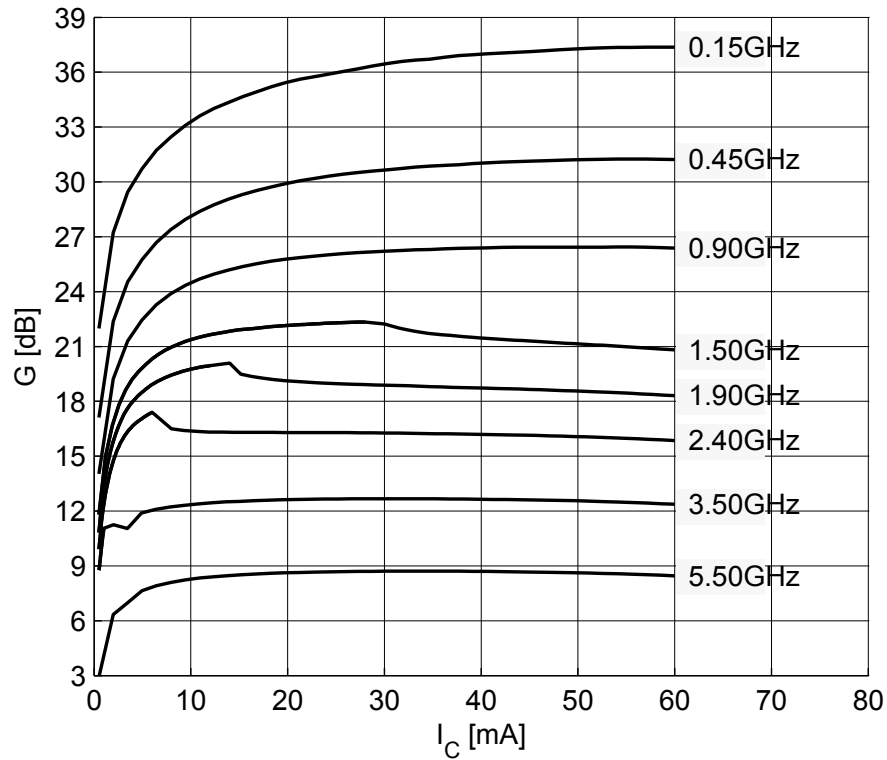
Figure 15 Maximum power gain G_{\max} = f(I_C) , V_{CE} = 3 \text{ V} , f = \text{parameter in GHz}
