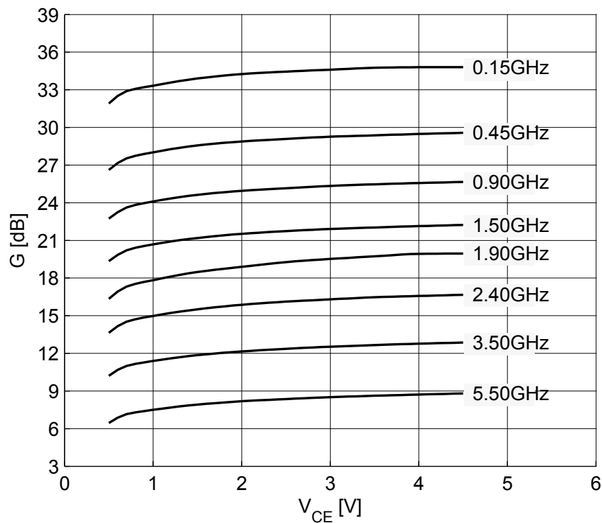
Figure 16 Maximum power gain G_{\max} = f(V_{CE}) , I_C = 15 \text{ mA} , f = \text{parameter in GHz}
