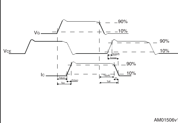
Figure 31. Switching waveform
