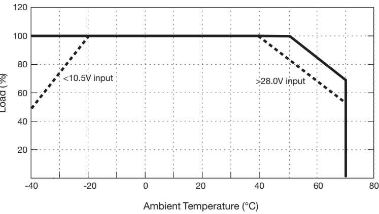
Derating curve
