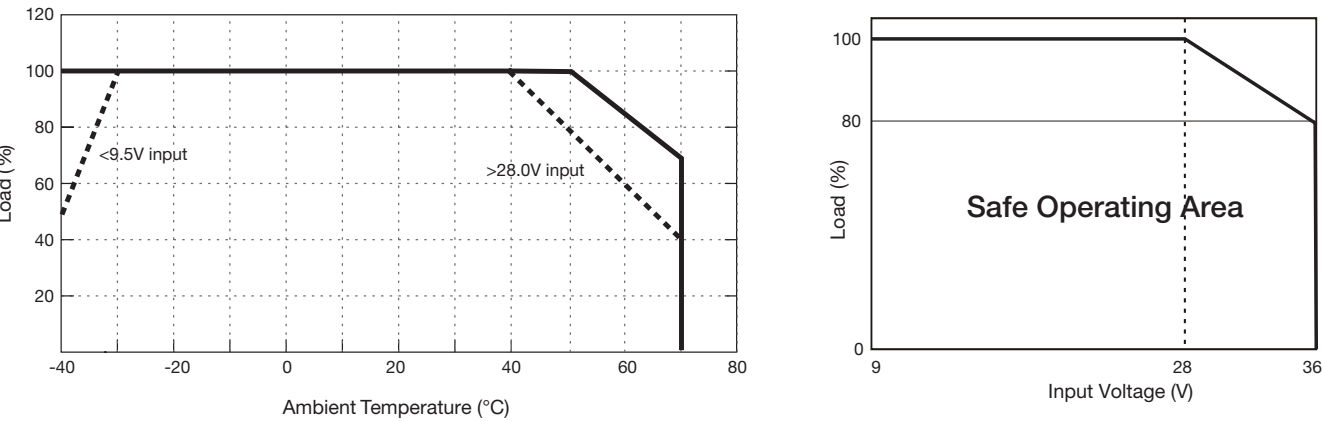
Derating curve
