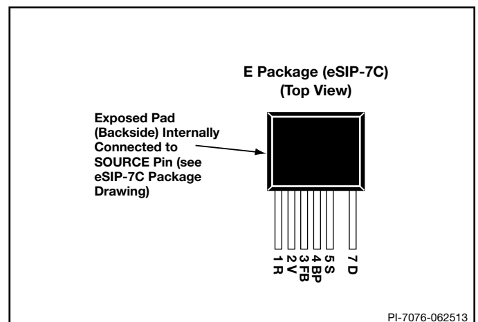
Figure 5. Pin Configuration.
