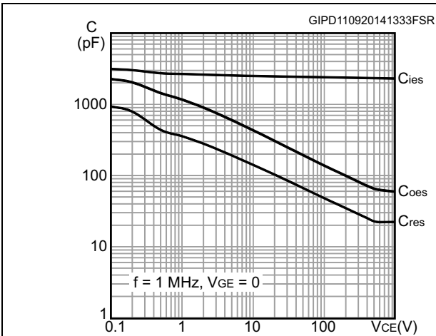
Figure 14. Capacitance variation
