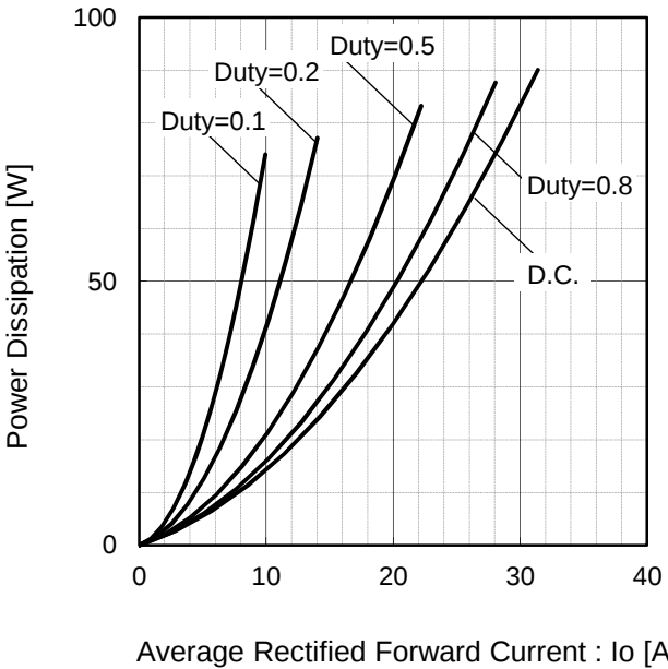
Fig.8 Io-Pf Characteristics
