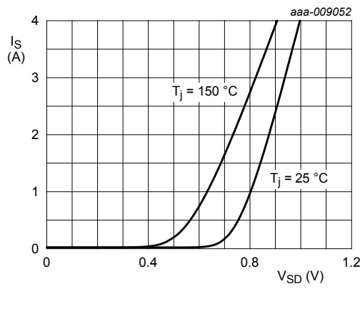
Fig. 16. Source current as a function of source-drain voltage; typical values
