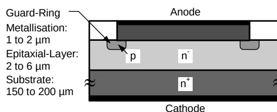
Fig 12. Schottky diode cross-section: The comprises of a metal alloy on a thin epitaxial layer. As for transistors the reverse side is electrically active.
