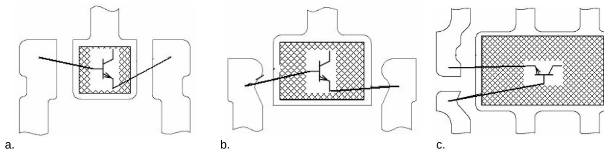
Fig 2. The standard lead frame of the SOT23 package (a.) limits the silicon area to about 0.5 \text{ mm}^2 . The lead frame of the SOT23 MaxSi (b.) permits to double the die area, and the SOT457 (c.) even provides a usable Si area of 1.85 \text{ mm}^2 .
