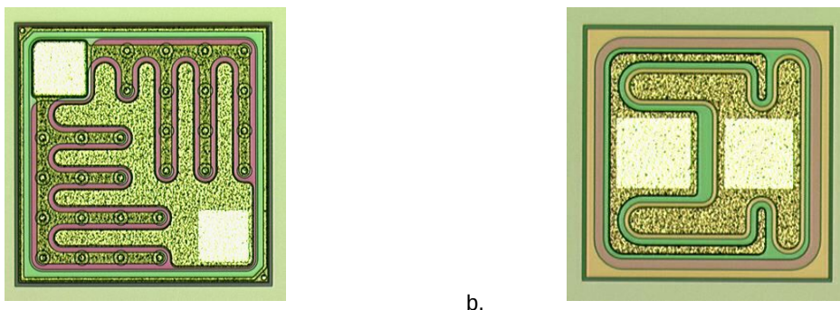
Fig 1. The die layout of a mesh-emitter transistor (a.) clearly shows the characteristic finger structure. Compared to the typical die layout of a conventional transistor (b.), a mesh-emitter transistor's finger structure and base contact holes provide a much larger active area.
