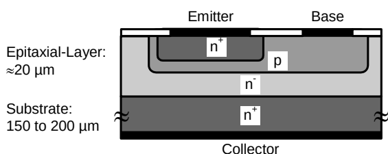
Fig 11. Bipolar transistor cross-section: The transistor is located in the epitaxial layer. As for diodes the much thicker substrate serves as carrier only.
