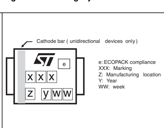
Figure 14. Marking layout (1)
