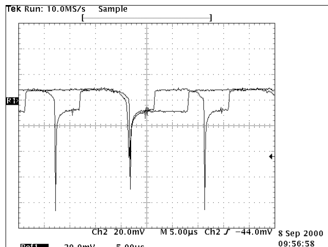
Figure 10-2: Base voltage of TR349
