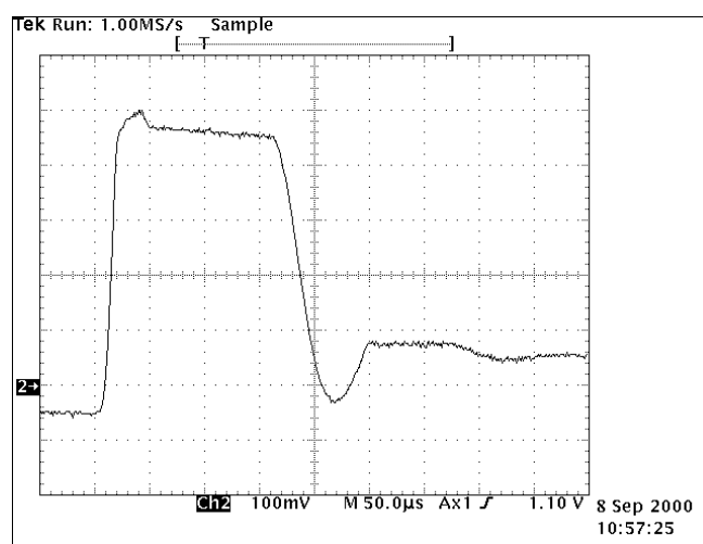
Figure 10-9: Vertical flyback voltage
