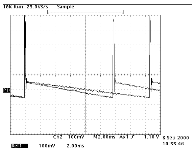
Figure 10-8: Vertical deflection output voltage
