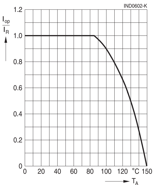
Current derating I_{\text{op}}/I_{\text{R}} versus ambient temperature T_{\text{A}} (rated temperature T_{\text{R}} = +85\text{ }^{\circ}\text{C} )
